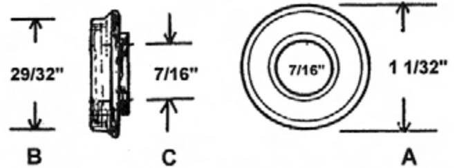
10X100 – INVACARE 8" WHEEL
