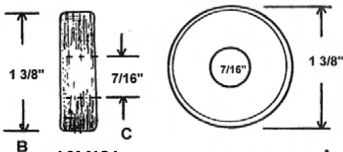
10X131 – INVACARE 24" WHEEL
