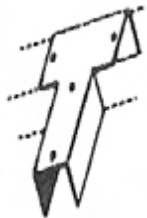
1175 T-BRACKET For suspended installations. Joins 2 tracks into 90 degree connection
