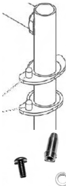
41X303- 1/4" Hanger Pin
